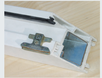
Plastic sections
